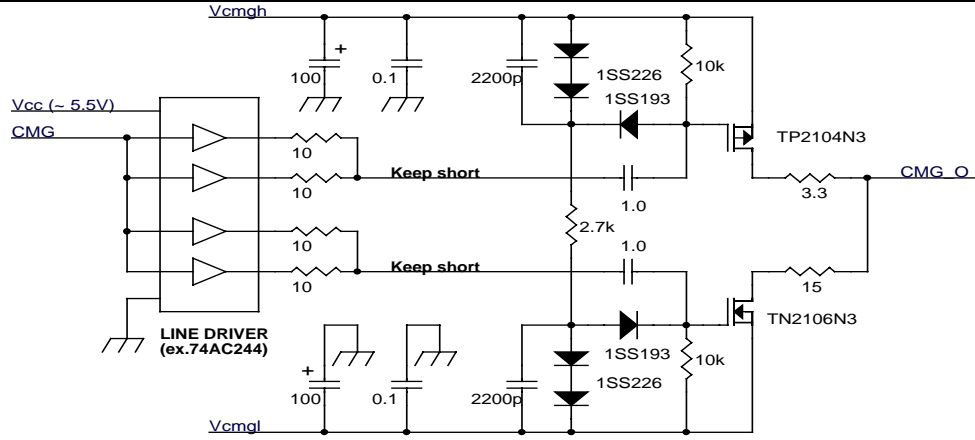
CMG Driver Circuit
